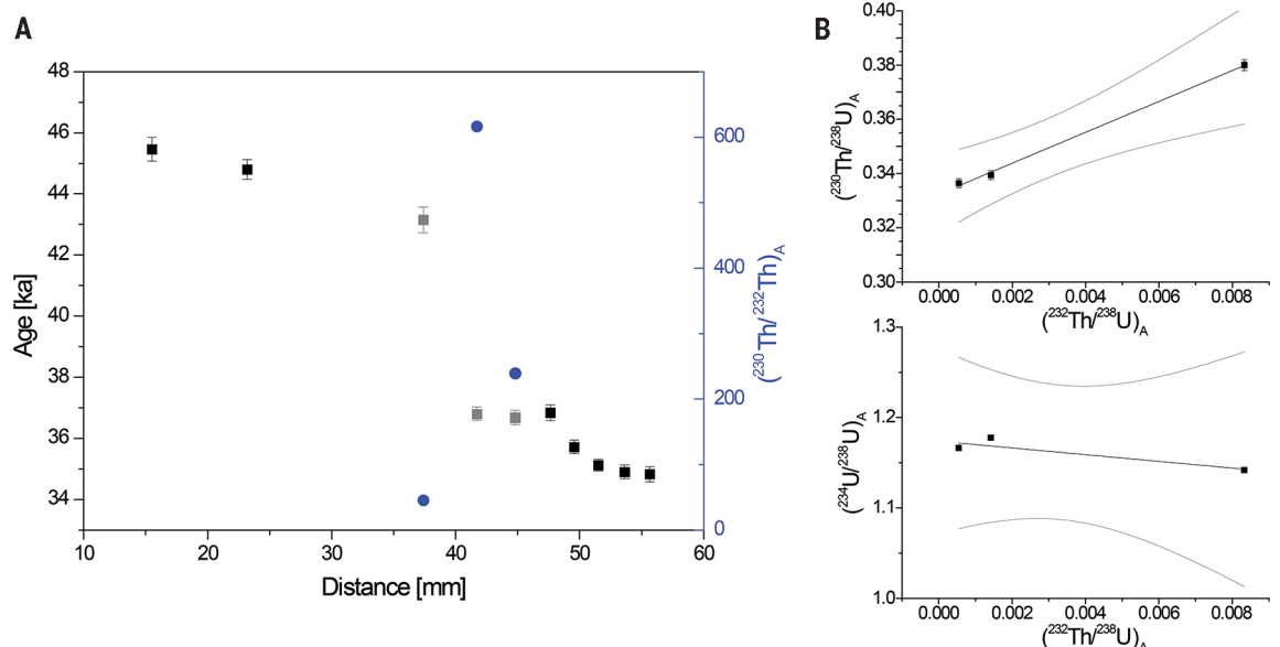
Fig. 1. A hypothetical example of erroneous isochron dating. (A) U-Th dating results across a 5-cm section of a flowstone (where distance is measured from the base). The results clearly reveal a 6-ka-long growth arrest at 40 mm.
