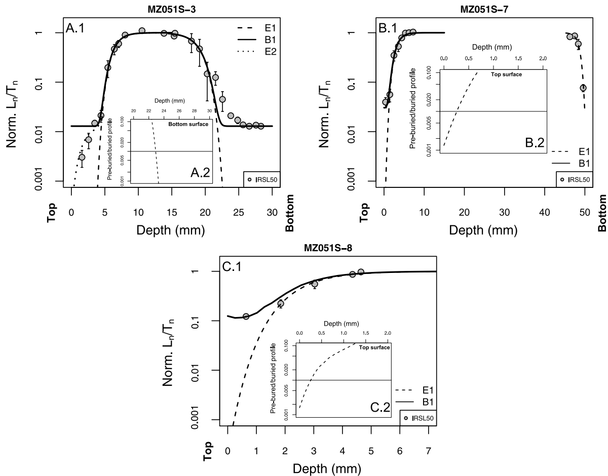
Fig. 7. Averaged (n≥2) IRSL 50 luminescence-depth profiles and their corresponding fits with the Freiesleben et al. (2015) model from MZ051S-3 (A), MZ051S-7 (B), and MZ051S-8 (C). The normalised sensitivity-corrected luminescence signals (L n /T n ) are plotted in logarithmic scale. The dashed lines in the insets show the ratios (E/B) between modelled exposure events (E) and modelled burial event (B) with depth.
