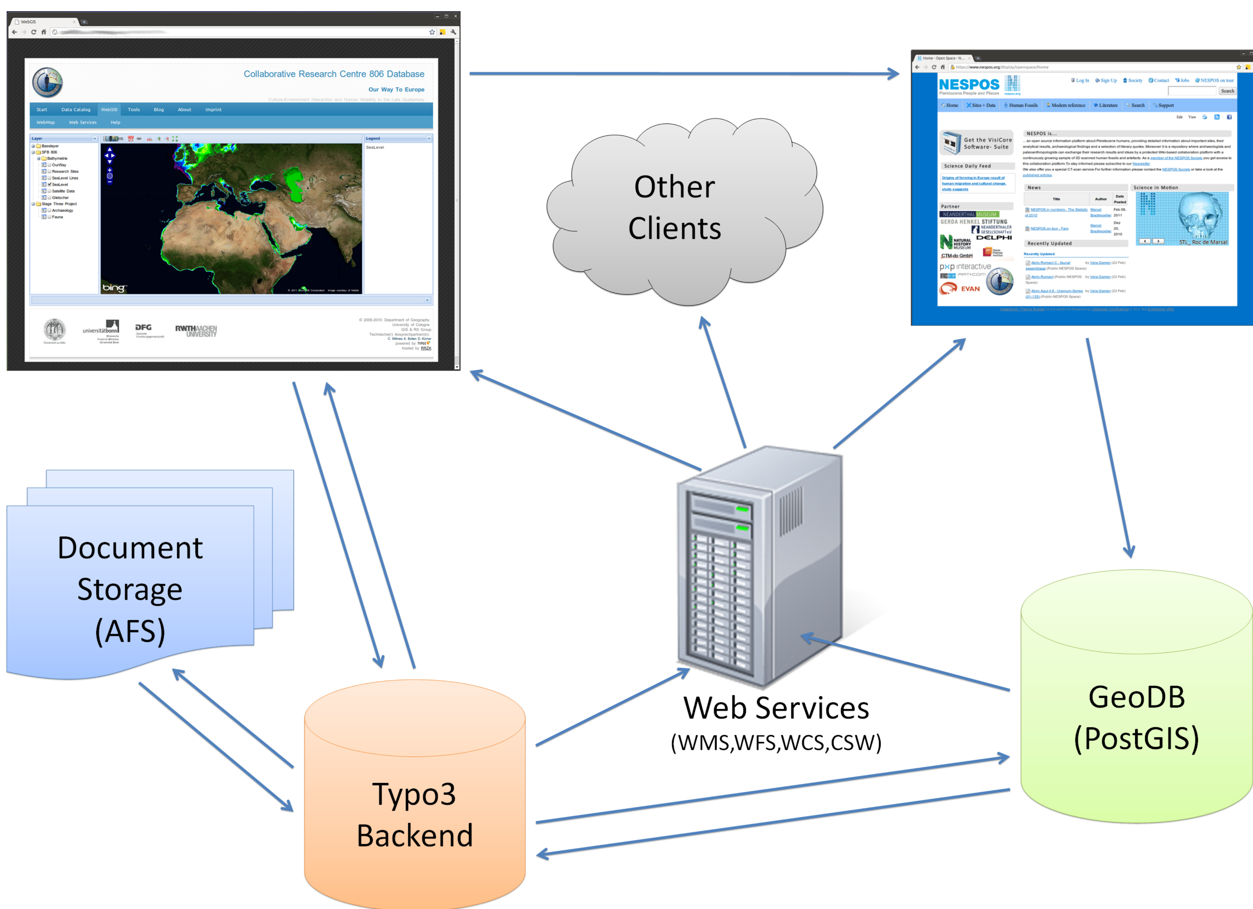
System architecture of the CRC806-Database data management infrastructure.
